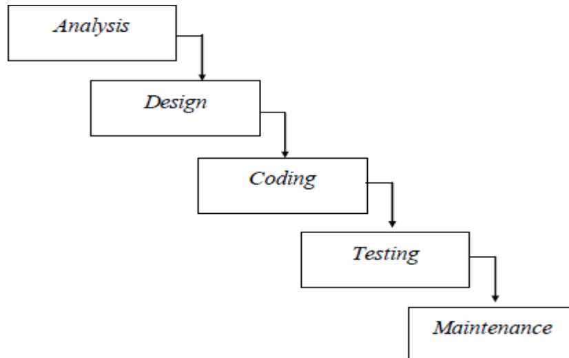
Gambar 2.3 Metode Waterfall
